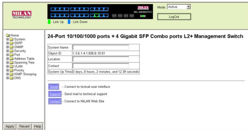
Figure 3-1 Home Page
